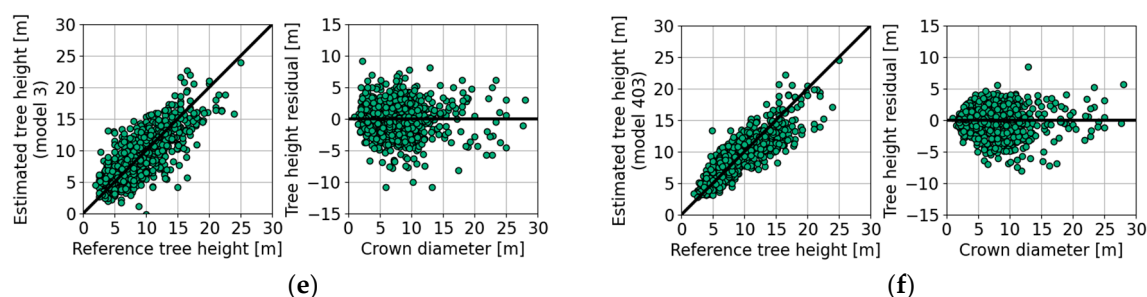
Figure 10. Tree height estimation performance for the selected best-performing models using: (a) TDM data only, (b) D_{avg} only, (c) d_{bh} only, (d) D_{avg} and d_{bh} , (e) TDM data and species information, (f) D_{avg} , d_{bh} , and species information. Mathematical expressions and estimation statistics are shown in Table 6. For (a–d), the models were fitted to data from all 915 trees, disregarding the species/genus of the trees. For (e,f), the models were fitted individually for each species/genus with at least ten times more trees than model parameters. In each panel, the first scatterplot from the left shows the estimated tree height ( \hat{h}_{top} ) on the y -axis against the reference tree height ( h_{top} ) on the x -axis, while the second scatterplot shows the obtained tree height residual ( h_{top} - \hat{h}_{top} ) against average canopy diameter ( D_{avg} ).
